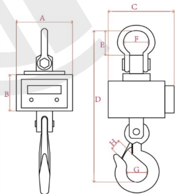
Electronic Dynamometer
